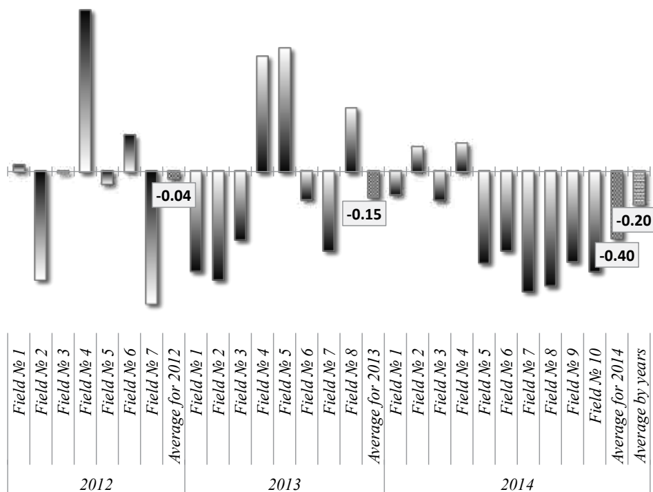
Fig. 2. Coefficients of correlation between the relative content of chlorophyll per unit area of the assimilative surface of winter wheat plants ( \text{mg}/\text{dm}^2 ) and NDVI
